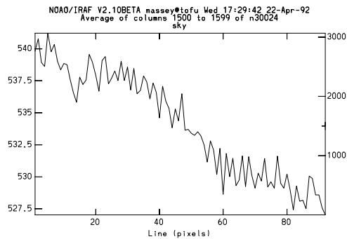
Figure 14: The cut along the spatial axis of a long program exposure appears to be consistent with a cut along the spatial axis of a bright twilight sky exposure: there is a 2% gradient from one side of the chip to the other.
