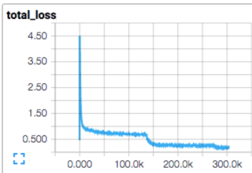
图 2.9: CIFAR-10 Loss
