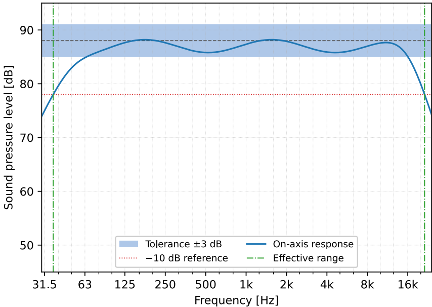
On-axis response
