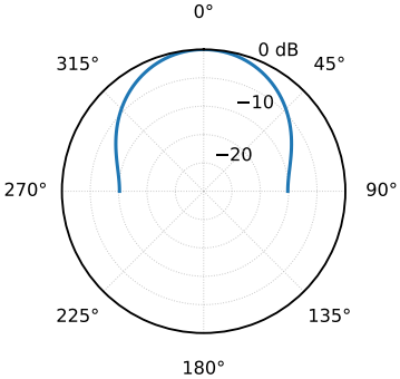
Directional response at 2000 Hz
