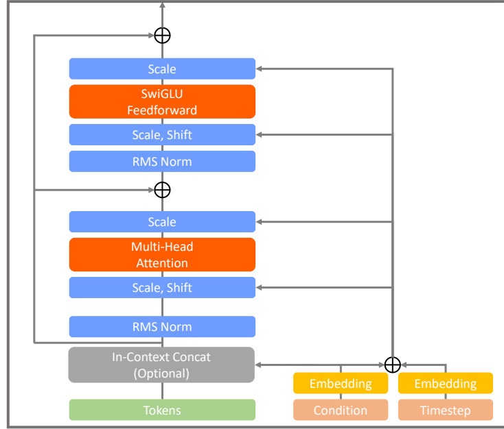
Fig. 8: Implementation of the JiT block. The in-context concatenation is operated only after the predefined in-context start block.
