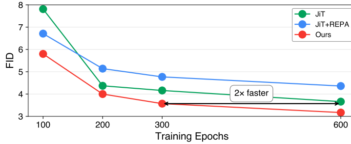
Fig. 1: REPA degrades JiT performance. As training progresses, JiT+REPA yields higher FID [14] ( \downarrow ) than vanilla JiT, indicating that REPA hinders pixel space diffusion training. PixelREPA prevents overfitting to the external semantic feature target, which accelerates convergence in JiT training. Remarkably, PixelREPA achieves > 2\times faster convergence than the vanilla JiT. All evaluated models utilize JiT-B/16.
