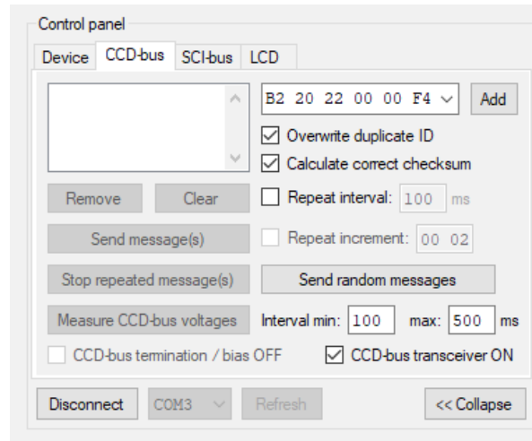
Figure 12. Controls on the CCD-bus tab.
