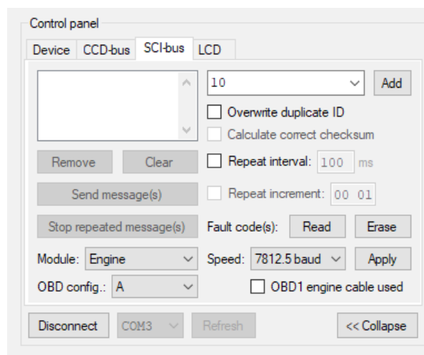
Figure 13. Controls on the SCI-bus tab.
