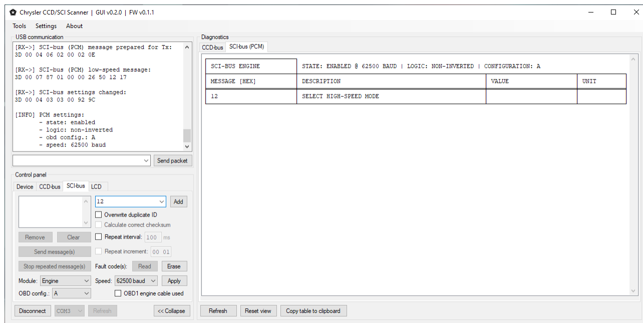
Figure 20. Switch SCI-bus to high-speed mode.
