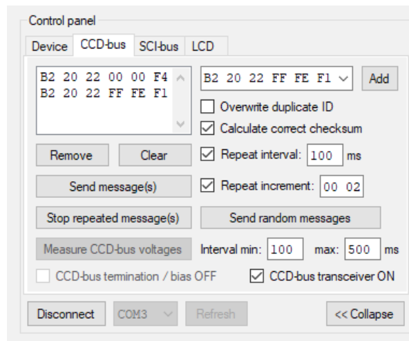
Figure 26. CCD-bus ROM reading example.
