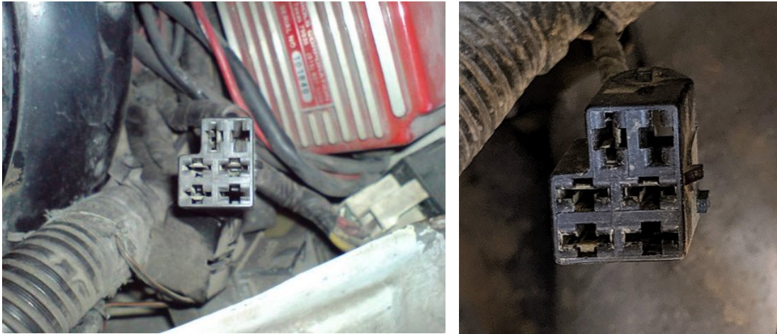
Figure 7. Engine connector (SCI-bus).
