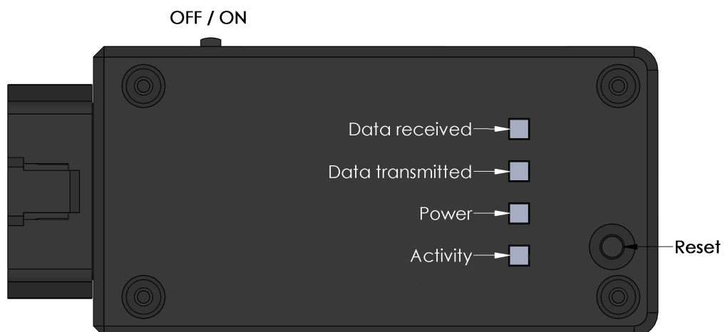
Figure 3. Status LED description and reset button location.
