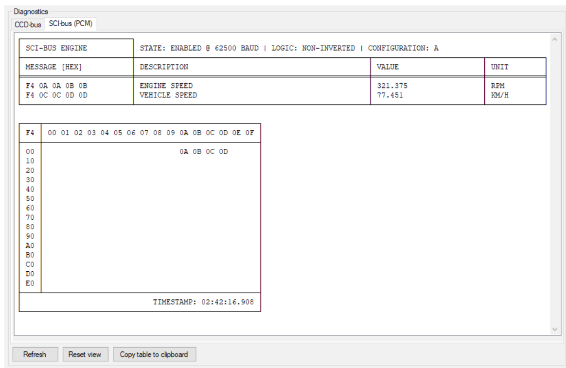
Figure 22. Custom high-speed SCI-bus request messages displayed in the table.
