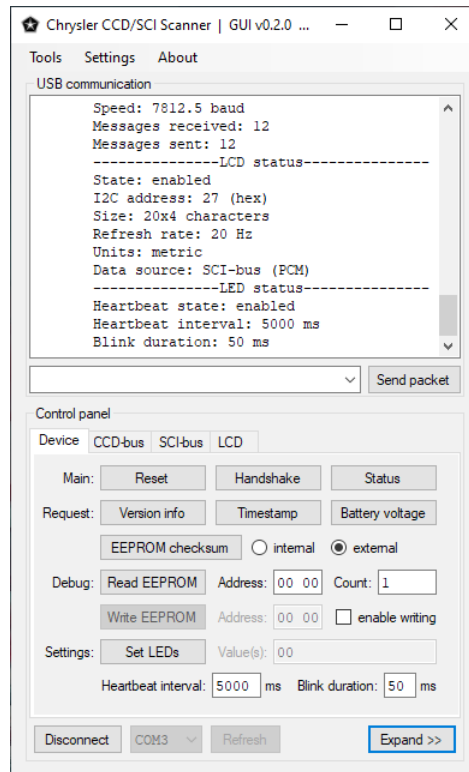
Figure 9. Windows GUI collapsed view.
