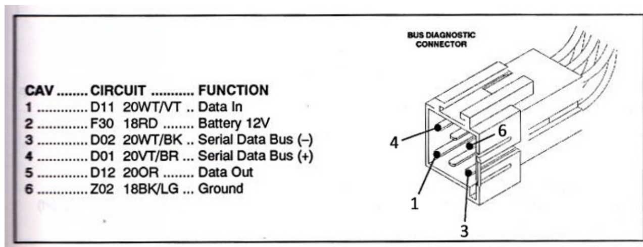
Figure 5. Body connector pinout.
