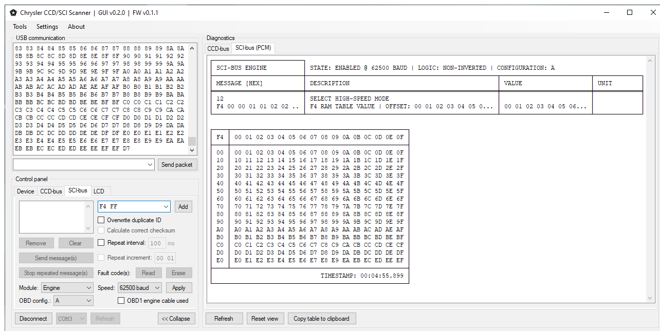
Figure 25. High-speed SCI-bus RAM table dump.
