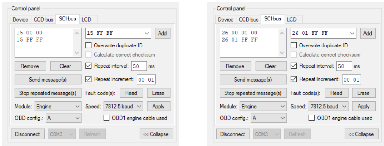
Figure 27. SCI-bus ROM reading example (left: 16-bit, right: 24 bit).
