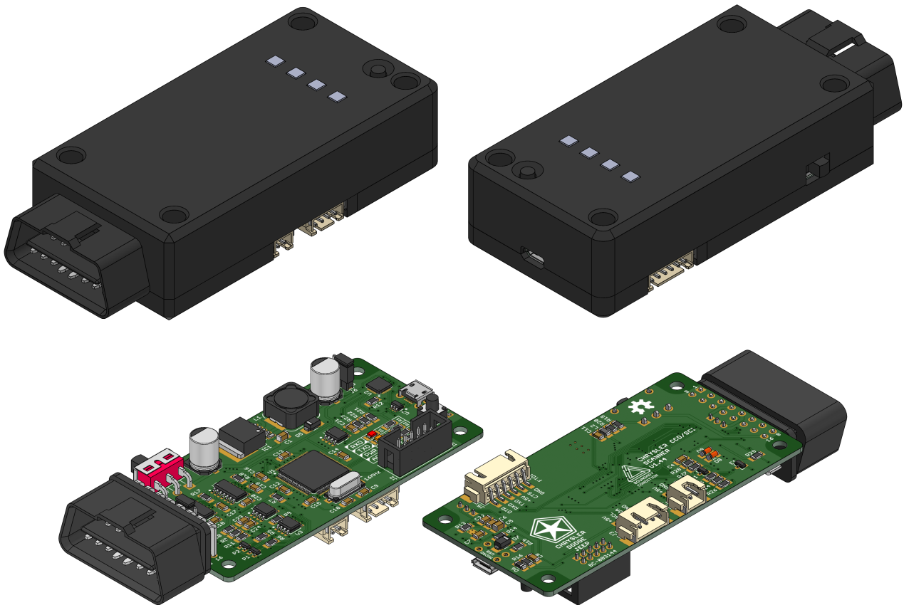
Figure 1. CAD drawing of the diagnostic scanner.
