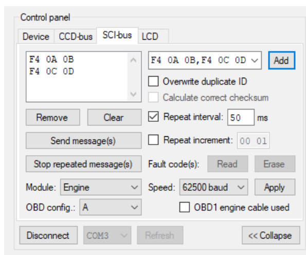
Figure 21. Custom high-speed SCI-bus request messages.
