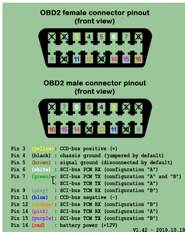
Figure 14. OBD2 connector pinout.
