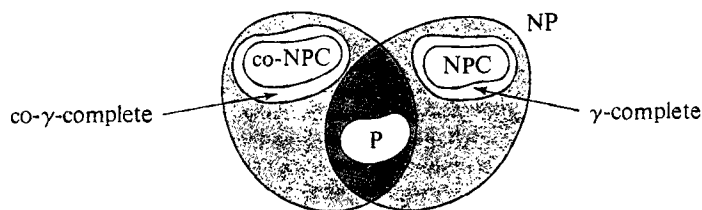
Figure 7.3 The world of NP, once more revised (assuming that both P \neq NP and NP \neq co-NP ).
