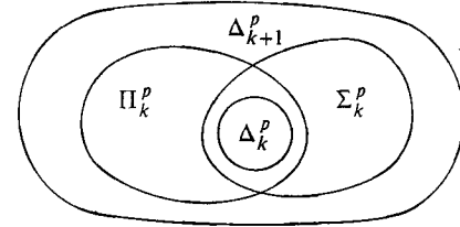
Figure 7.5 Containment relationships within the polynomial hierarchy.
