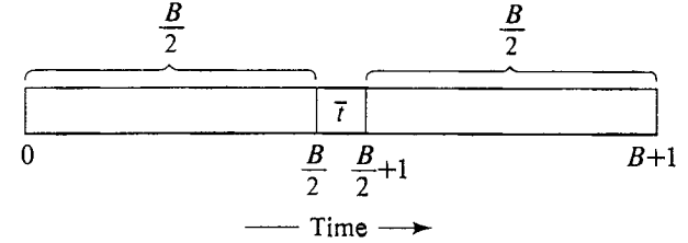
Figure 3.9 Schedule “enforced” by the transformation from PARTITION to SEQUENCING WITHIN INTERVALS.
