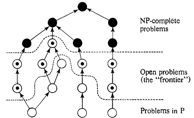
Figure 4.2 One possible state of knowledge about subproblems of an NP-complete problem \Pi . Problems are represented by circles, filled-in if known to be NP-complete, empty if known to be in P, and dotted if “open.” An arrow from \Pi_1 to \Pi_2 signifies that \Pi_1 is a subproblem of \Pi_2 .
