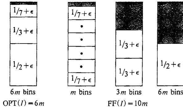
Figure 6.2 Instances I with \text{OPT}(I) arbitrarily large such that \text{FF}(I) equals (5/3)\text{OPT}(I) .
