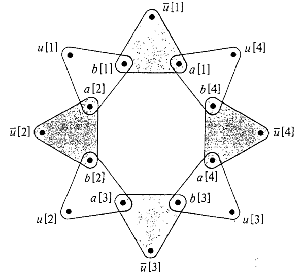
Figure 3.2 Truth setting component T_i when m = 4 (subscripts have been deleted for simplicity). Either all the sets of T_i (the shaded sets) or all the sets of T_i' (the unshaded sets) must be chosen, leaving uncovered all the u_i[j] or all the \bar{u}_i[j] , respectively.
