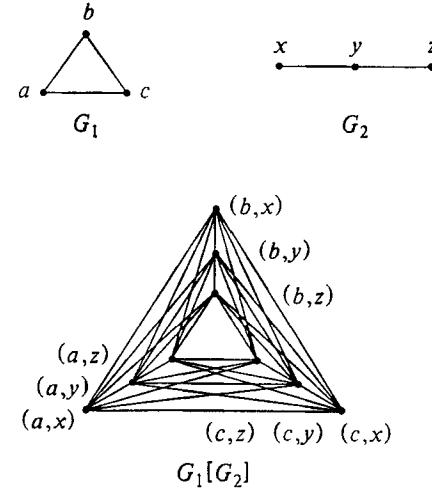
Figure 6.6 The composition G_1[G_2] of two graphs G_1 and G_2 .
