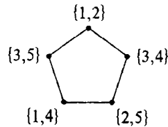
Figure 6.7 A (5, 2) -multicoloring of a pentagon C_5 , with each vertex v labeled by the corresponding set f(v) of “colors.” It can be shown that \chi_2(C_5) = 5 .
