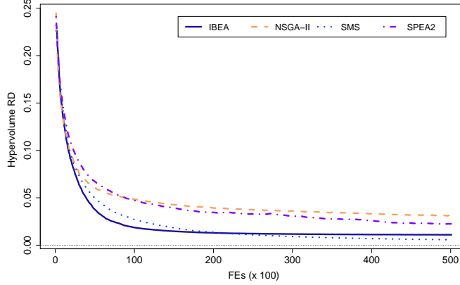
Figure 4: Mean I_H^{\text{rd}} values of different MOEAs using parameter settings tuned for a common stopping criterion ( FE_{\text{max}} = 10\,000 ) on WFG3 ( M = 3 , n_{\text{var}} = 50 ).
