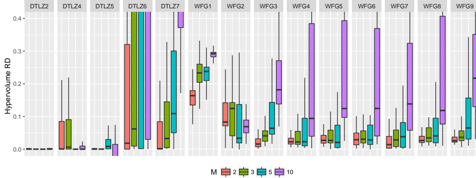
Figure 7: Boxplots of all I_H^{\text{rd}} values for FE_{\max} = 10000 , grouped by M and benchmark function, depicting how dominance resistance affects problems in different ways.
