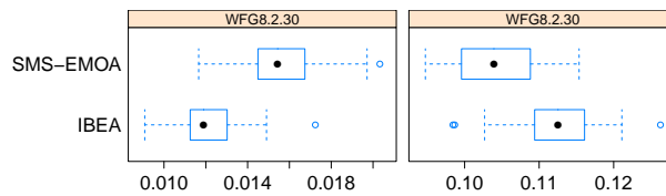
Figure 5: SMS and IBEA performance according to the I_H^{\text{rd}} (left) and IGD (right) on function WFG8 ( M = 2 , n_{\text{var}} = 30 , FE_{\max} = 10\,000 ).
