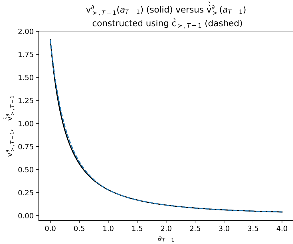
Figure 10 True v_{>(T-1)}^\partial(a) vs. \hat{v}_{>(T-1)}^\partial(a) Constructed Using \hat{c}_{>(T-1)}(a)
