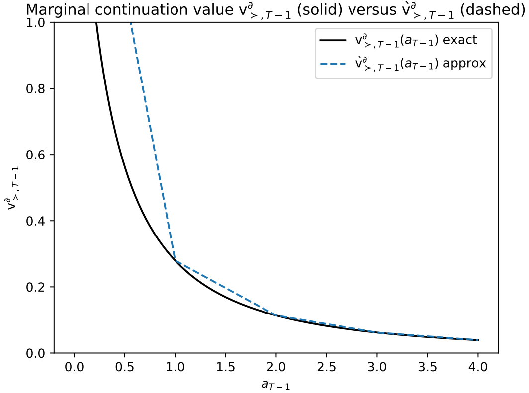
Figure 7 v_{>(T-1)}^{\partial}(a_{T-1}) versus \hat{v}_{>(T-1)}^{\partial}(a_{T-1})
