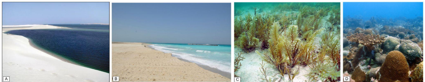
Habitats in the modern Persian Gulf that are likely similar to the Michigan Basin during the Silurian. A. super-tidal dunes, B. inter-tidal beach, C. algae beds, and D. coral reefs. Images from Vaughan, Grace O., Noura Al-Mansoori, and John A. Burt. "The arabian gulf." World seas: An environmental evaluation. Academic Press, 2019. 1-23.
