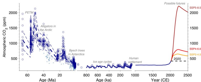
Atmospheric CO 2 since the Dinosaur extinction. Note that the time scale changes along the x-axis. Atmospheric CO 2 is now present in our atmosphere at higher levels than it has been since the beginning of the ice age 2.58 million years ago. From Rae et al., (2021)
