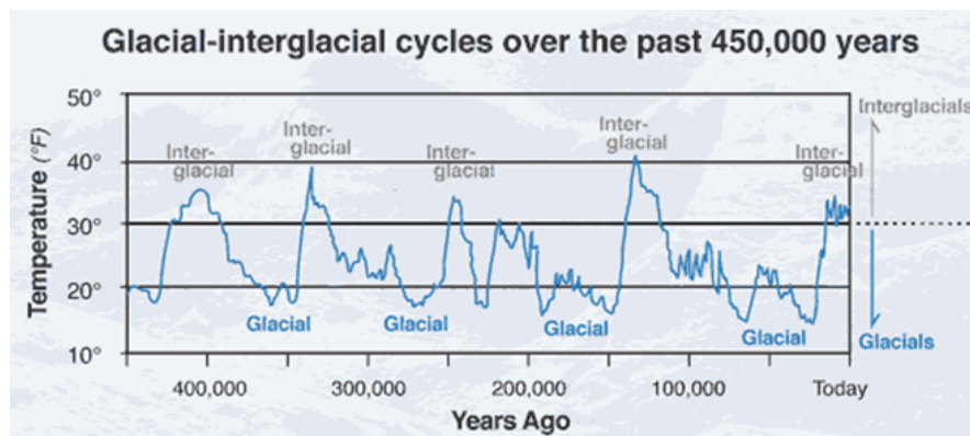
Global average air temperature for the last 500,000 years (0.5 Ma). Image from: https://geology.utah.gov/map-pub/survey-notes/glad-you-asked/ice-ages-what-are-they-and-what-causes-them/
