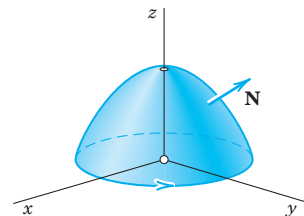
Fig. 255. Surface S in Example 1
