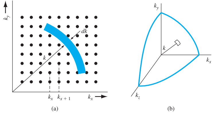
Figure 3.26 | (a) A two-dimensional array of allowed quantum states in k space. (b) The positive one-eighth of the spherical k space.
