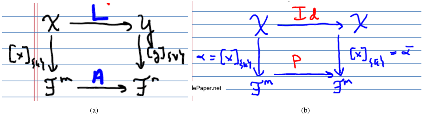
Figure 2.1: Diagram chasing. Commuting diagrams used to illustrate the matrix representation of a linear operator and the change of basis matrix. When \mathcal{X} = \mathcal{Y} and \mathcal{L} = Id , they become one and the same. Hence, there is really only one idea to remember.
