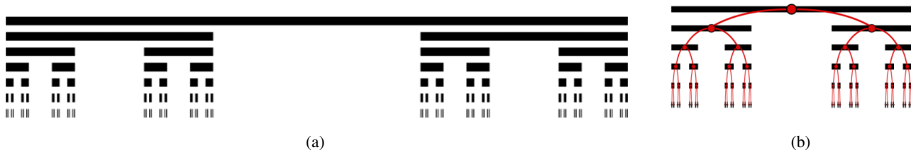
Figure 5.1: Images of the Cantor set, thanks to Wikipedia. (a) The top line is the interval [0, 1] . The line below is what is left when one removes the (open) middle third, (1/3, 2/3) . The line below that is what is left when the next two (open) middle thirds, (1/9, 2/9) and (7/9, 8/9) , are removed, etc. In the beginning, it's hard to believe that there is anything left over, but there is. In fact, the Cantor set can be placed in one to one correspondence with the original interval [0, 1] . (b) Shows various paths traced out in a ternary (base 3) expansion of numbers in the Cantor set; “each point in the Cantor set is uniquely located by a path through an infinitely deep binary tree, where the path turns left or right at each level according to which side of a deleted segment the point lies on. Representing each left turn with 0 and each right turn with 2 yields the ternary [expansion] for a point”, from Wikipedia https://en.wikipedia.org/wiki/Cantor_set . Replacing the 2's with 1's yields a bijection from the Cantor set to the interval [0, 1] , which is cool and surprising, though otherwise irrelevant to ROB 501!
