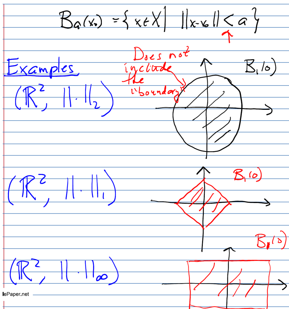
Figure 6.1: (\mathbb{R}^2, \|\bullet\|) with various norms: (a) Euclidean norm \|(x_1, x_2)\|_2 = \sqrt{|x_1|^2 + |x_2|^2} ; (b) One norm \|(x_1, x_2)\|_1 = |x_1| + |x_2| ; and (c) Max norm \|(x_1, x_2)\|_\infty = \max_{1 \leq i \leq 2} |x_i| .
