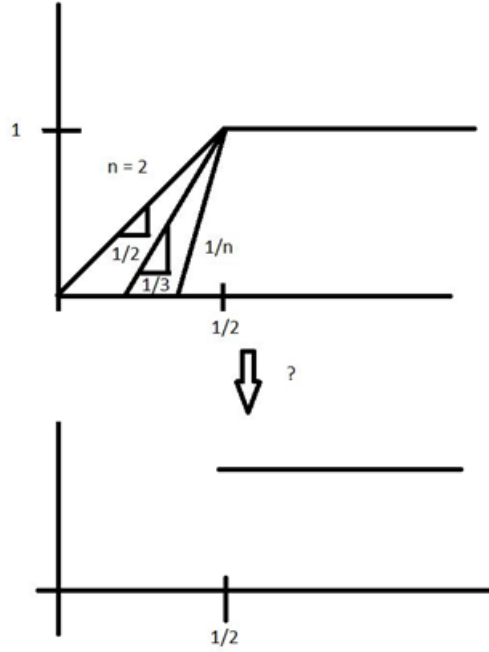
Figure 6.3: Visually, the sequence of continuous functions (f_n(t))_{n=2}^{\infty} appears to be converging to a step function, which is discontinuous. If that is true, we then have a Cauchy sequence in (\mathcal{X}, \|\bullet\|_1) that does not have a limit in the set \mathcal{X} .
