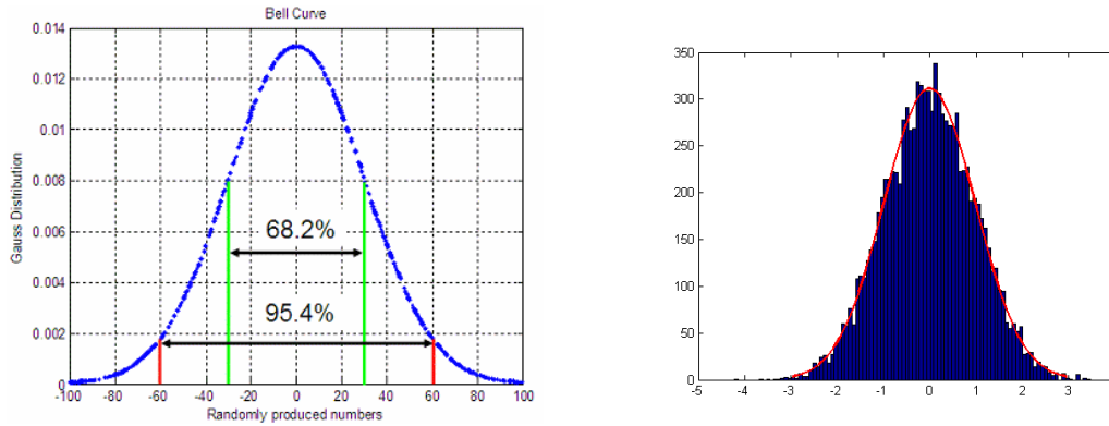
Figure 5.2: (Left) Normal distribution N(\mu, \sigma) with \mu = 0 and \sigma = 30 . (Right) How do you determine the density? You have to collect data! The figure shows a “fit” of a normal distribution to data.
