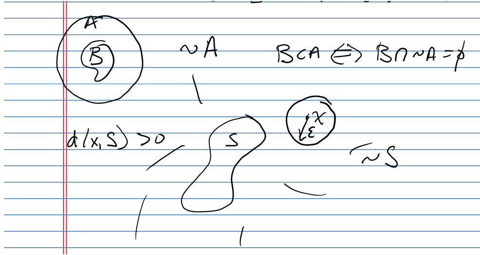
Figure 6.2: Why (d(x, S) > 0) \iff (\exists \epsilon > 0 \text{ such that } B_\epsilon(x) \subset (\sim S)) \iff (\exists \epsilon > 0 \text{ such that } B_\epsilon(x) \cap S = \emptyset) . We simply take \epsilon = \frac{d(x, S)}{2} > 0 .
