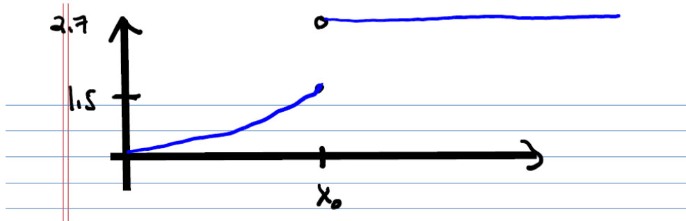
Figure 6.4: Let \epsilon = 1.0 Then, \forall \delta > 0, \exists x \in B_\delta(x_0) such that |f(x) - f(x_0)| \geq \epsilon . Indeed, x = x_0 + \delta_2 works.
