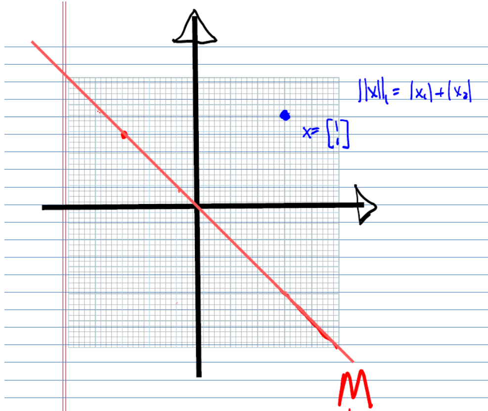
Figure 3.1: In HW, we'll introduce the concept of “strict” norms. The \|\bullet\|_1 is not strict and consequently, the minimum distance problem (or best approximation problem) does not have a unique answer.
