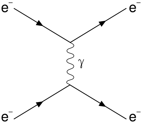
'CC BY-SA 4.0' 'Electron-scattering.svg' see 'ATtribution' Feynman diagram of *virtual* photon, exchange of which can account for electrical and/or magnetic repulsion and/or attraction.
