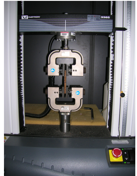
'Tensile testing on a coir composite.jpg' see 'ATtribution'
