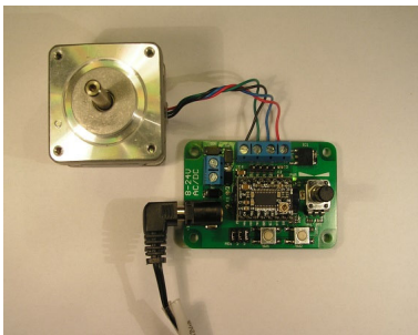
EasyStepper from reprap.org
