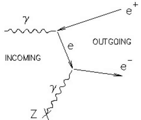
'Electron-Positron nuclear Pair production Feynman Diagram.gif' see 'ATtribution'
