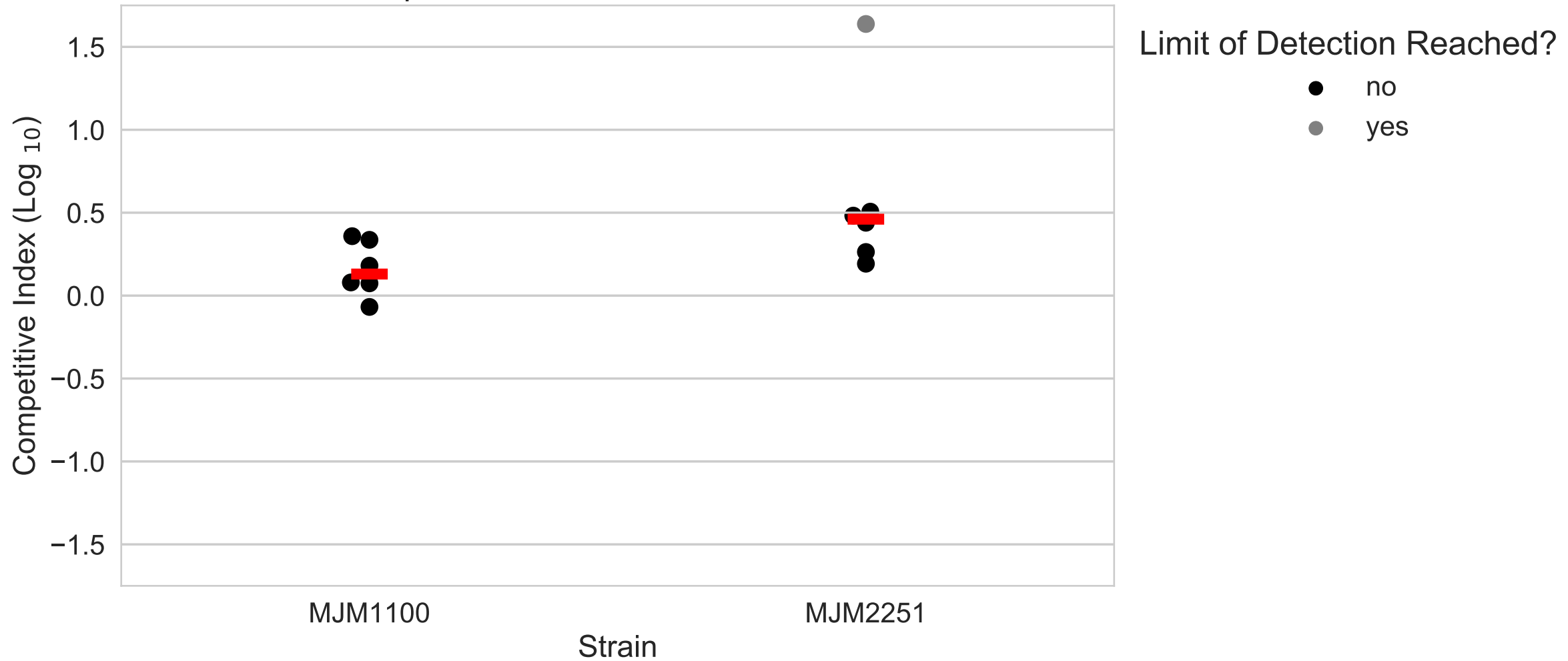
Competitive Index of Strains vs ES114
