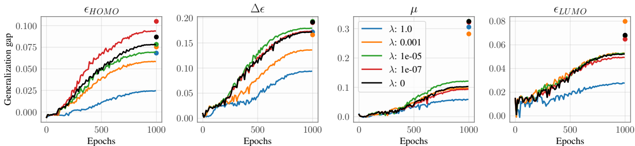
Figure 5. Generalization gap over training epochs for the regularization method proposed in this work. Circles at the end of training denote the final test MSE error.
