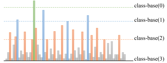
Figure 1. Structure of RobustSL having four classes. Items in lower-indexed classes replicate more. The replication of items within a class is achieved through a stochastic process.
