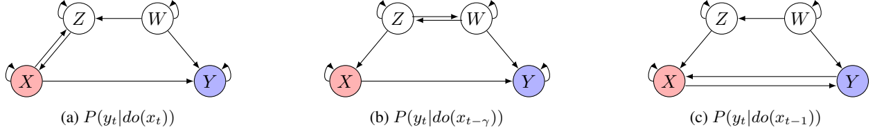
Figure 5.1: Three SCGs and a total effect which is identifiable. Each pair of red and blue vertices in the FTCGs represents the total effect we are interested in, and we precise the total effect and the lag considered in the caption. This illustrates Lemma 5.2 (Figure a-b) and Lemma 5.3 (Figure c).
