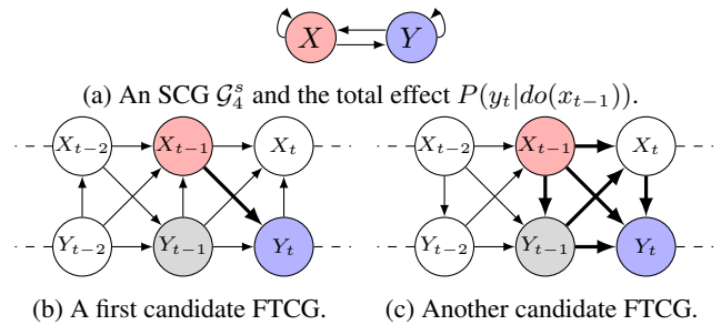
Figure 5.5: An example of an SCG \mathcal{G}_4^s in (a) satisfying Condition 2c in Theorem 2 with respect to \Pr(y_t | do(x_{t-1})) and two candidate FTFCGs in (b) and (c). Each pair of red and blue vertices in the FTFCGs represents the total effect we are interested in. Gray vertices are ambiguous: they constitute a backdoor path in (b) and belong to a directed path in (c) (bold edges indicate direct paths from X_{t-1} to Y_t ).
