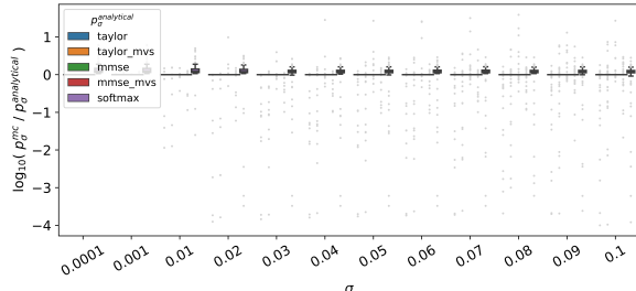
(h) CIFAR100, Vision Transformer
