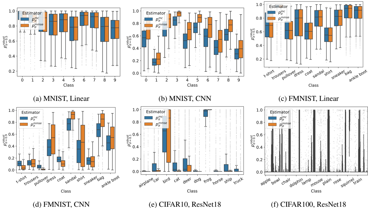
Figure 13: Local robustness bias among classes. p_{\sigma}^{\text{robust}} reveals that the model is less locally robust for some classes than for others. The analytical estimator p_{\sigma}^{\text{mmse}} properly captures this model bias.
