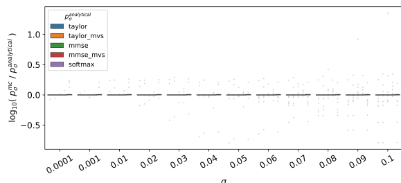
(g) CIFAR10, Vision Transformer
