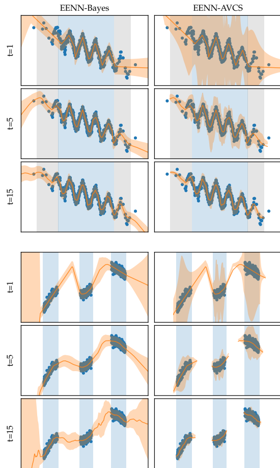
Figure 3: Prediction intervals (■) for EENN-Bayes ( left ) and our EENN-AVCS ( right ) on two simulated regression tasks \mathcal{?} : wiggle ( up ) and 3-clusters ( bottom ). Blue points denote training data. In cases where the EENN-AVCS collapses to an empty set (out-of-distribution), we do not depict anything, which explains the gaps in EENN-AVCS predictions. We set the significance level to \alpha = 0.05 for EENN-AVCS, while for EENN-Bayes, we plot intervals that capture 2 standard deviations away from the predicted mean (—). With different background colors we denote different regions of data distribution, see Section 7.1.
