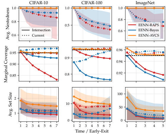
Figure 6: Comparison of our EENN-AVCS with RAPS [?] and EENN-Bayes baselines based on average nestedness ( top ), marginal coverage ( middle ), and average interval size ( bottom ) for our image classification experiments using MSDNet as a backbone. EENN-AVCS is the only approach that attains perfect nestedness ( top ) while maintaining high marginal coverage across different exits ( middle ). Nestedness comes at a price, though, as EENN-AVCS sets are larger compared baseline ones ( bottom ). Note that in the top plot, the nestedness curves of EENN-AVCS (—), RAPS-intersection (—), and EENN-Bayes -intersection (—) overlap at \mathfrak{N}(t) = 1 .
