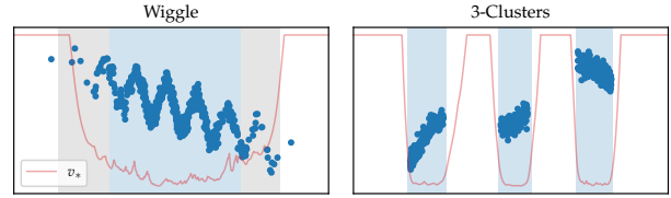
Figure 4: Average epistemic uncertainty v_* ( \text{---} ) across Bayesian linear regression models at different exits. As expected, v_* is larger in the regions where we observe less training data: out-of-distribution (denoted with a white background) and in-between (denoted with a grey background \blacksquare ). Hence, v_* can serve as an indicator for assessing the reliability of EENN-AVCSs.
