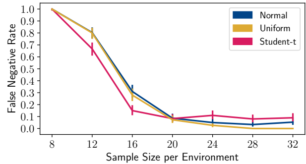
Figure 2: The behavior of the false negative rate of L-ICP under a misspecified noise model.
