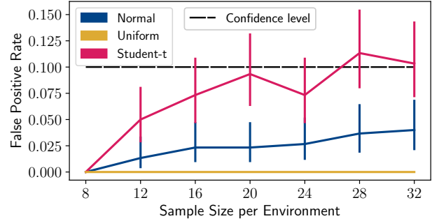
Figure 1: The behavior of the false positive rate of L-ICP under a misspecified noise model.
