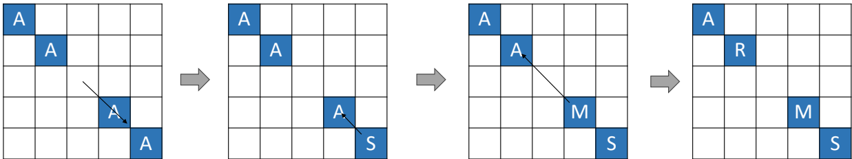
Figure 4: Acronym
