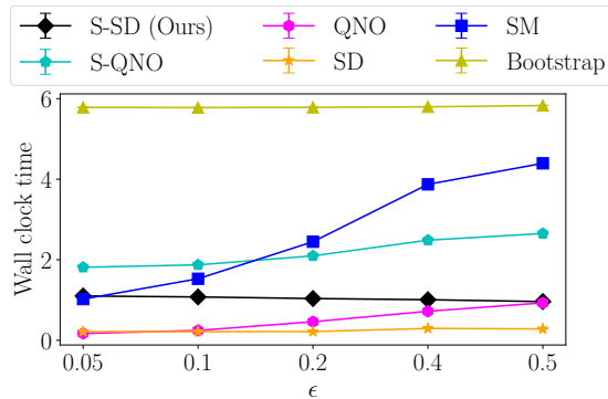
Figure 2: Computational efficiency: x -axis shows the value of \epsilon , y -axis shows the wall clock time in seconds. Our basic (non-stepwise) approach
