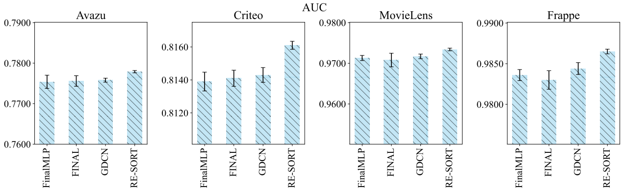
Figure 5: Variance comparison of different SOTA models.
