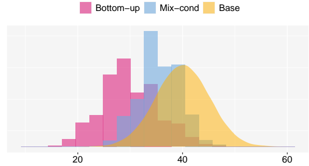
Figure 2: Predictive distribution of U : bottom-up (discrete), reconciled (mix-cond, discrete) and base (Gaussian).
