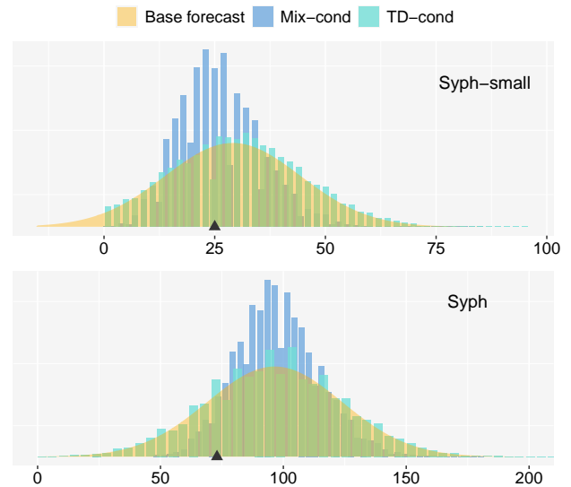
Figure 7: Base forecasts, reconciled distributions ( Mix-cond , TD-cond ), and actual values (black triangles) for Syph-small and Syph dataset.
