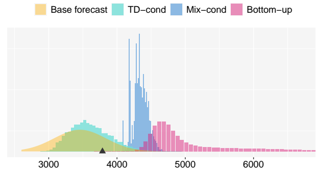
Figure 3: Predictive distribution for the top time series ( M5 dataset, store WI_1 ): base ( \hat{\pi}_U , Gaussian), reconciled (TD-cond and Mix-cond), and bottom-up ( \hat{\pi}_{bu} , discrete). The black triangle is the actual value.
