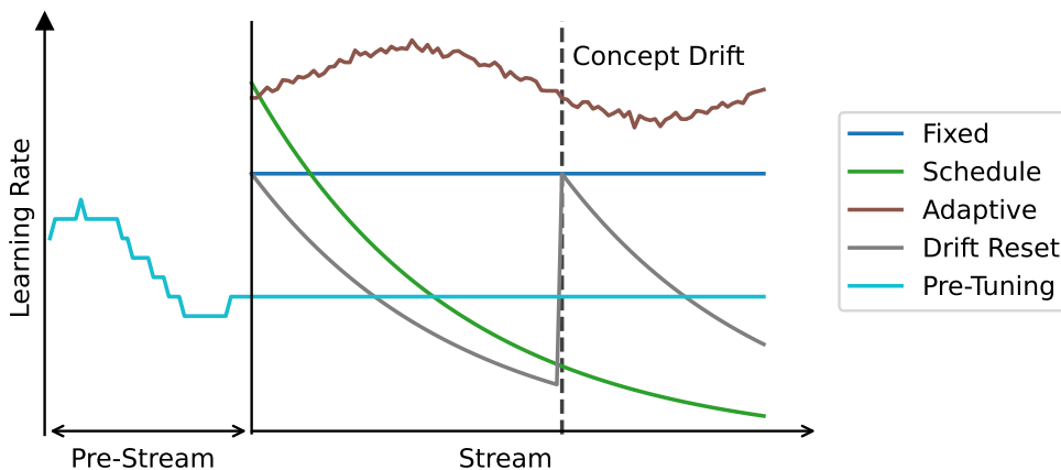
Figure 1: Overview of different learning rate optimization approaches.
