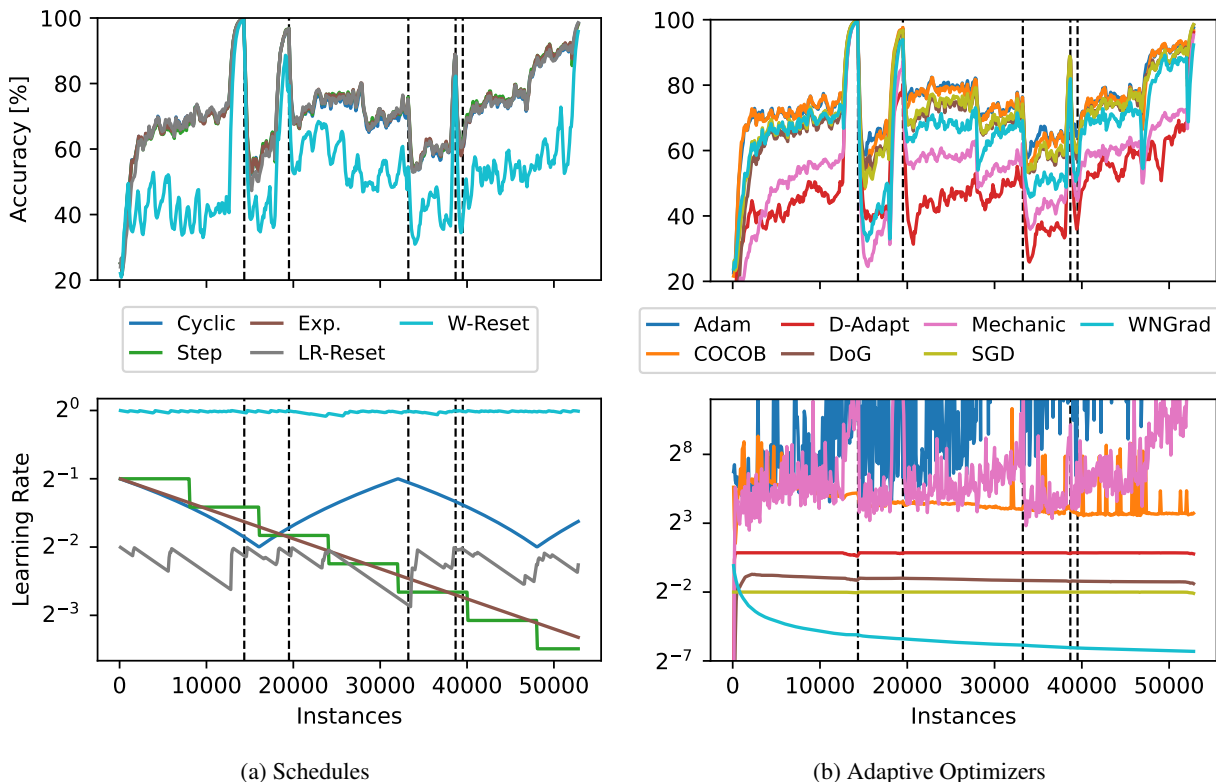
Figure 2: Prequential accuracy and learning rate for different schedules and adaptive optimizers on Insect a dataset. Concept drifts are marked by dashed lines. Accuracy is exponentially smoothed with a decay factor of 0.75. Note that the learning rates of COCOB, Adam, and Mechanic in b are much larger compared to DoG etc. due to being scaled by an estimate of the second-moment of past gradients.
