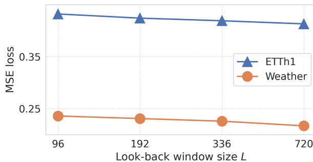
Figure 11: The forecasting performance on ETTh1 and Weather datasets, across 4 different look-back window sizes. The prediction length was fixed as T = 336 .
