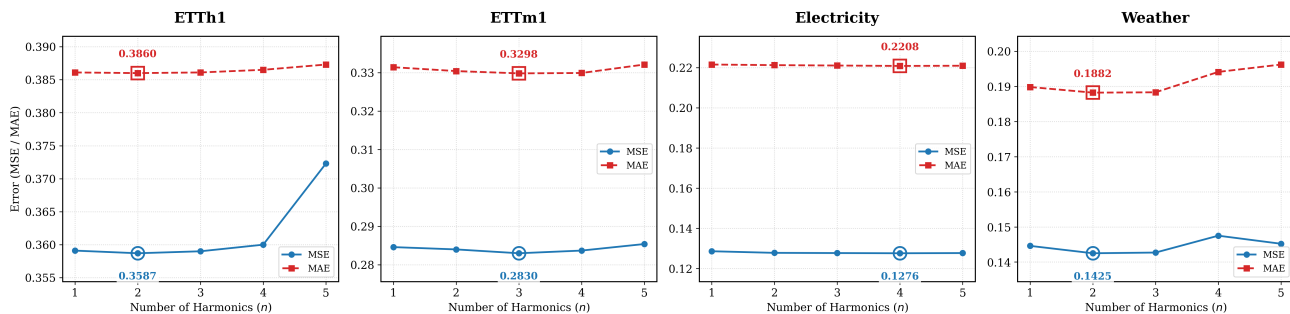
Figure 10: Performance comparison w.r.t different number of harmonics n on four datasets.
