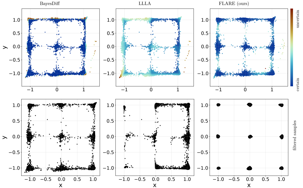
Figure 4: DDIM - Mode interpolation on a 2D Gaussian mixture adapted from Aithal et al. (2024) and Jazbec et al. (2025). The dataset consists of 9 Gaussian modes arranged on a square grid. The top row shows uncertainty scores from BayesDiff (left), LLLA (middle), and our method (right) for generated samples. The bottom row shows the same generated samples after filtering by a fixed uncertainty threshold. BayesDiff fails to assign high scores to points between modes, while LLLA performs even worse, leading to unreliable filtering. In contrast, our method produces faithful uncertainty estimates, enabling consistent removal of low-confidence samples.
