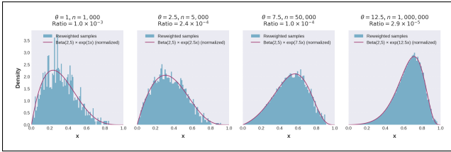
Figure 3: Exponential tilting of Beta(2, 5) distribution with a sequence of (\theta_i, n_i) s.t. M_{\theta}/n \rightarrow 0 .
