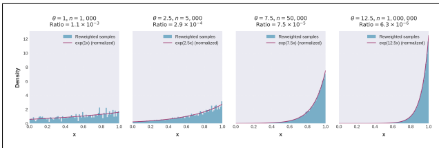
Figure 5: Exponential tilting of Uniform(0, 1) distribution with a sequence of (\theta_i, n_i) s.t. M_{\theta}/n \rightarrow 0 .
