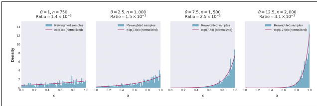
Figure 4: Exponential tilting of Uniform(0, 1) distribution with a sequence of (\theta_i, n_i) s.t. M_{\theta}/n \not\rightarrow 0 .
