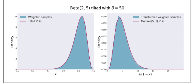
Figure 6: Exponential tilting of Beta(2, 5) distribution with \theta = 50 . The PDF of the samples and true distribution is on the left. The transformed samples, given in Theorem 5, with the PDF of \Gamma(5, 1) , the corresponding scaling limit.
