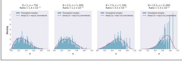
Figure 2: Exponential tilting of Beta(2, 5) distribution with a sequence of (\theta_i, n_i) s.t. M_{\theta}/n \not\rightarrow 0 .
