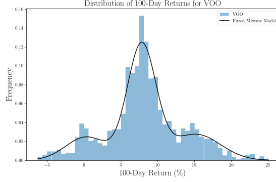
Figure 5: Real-world motivation for bandits with mixture distributions: Multimodal distribution of 100-day returns for VOO (a financial stock), showing the observed histogram of returns (blue bars) and a fitted mixture model (black curve) capturing the multimodal structure.
