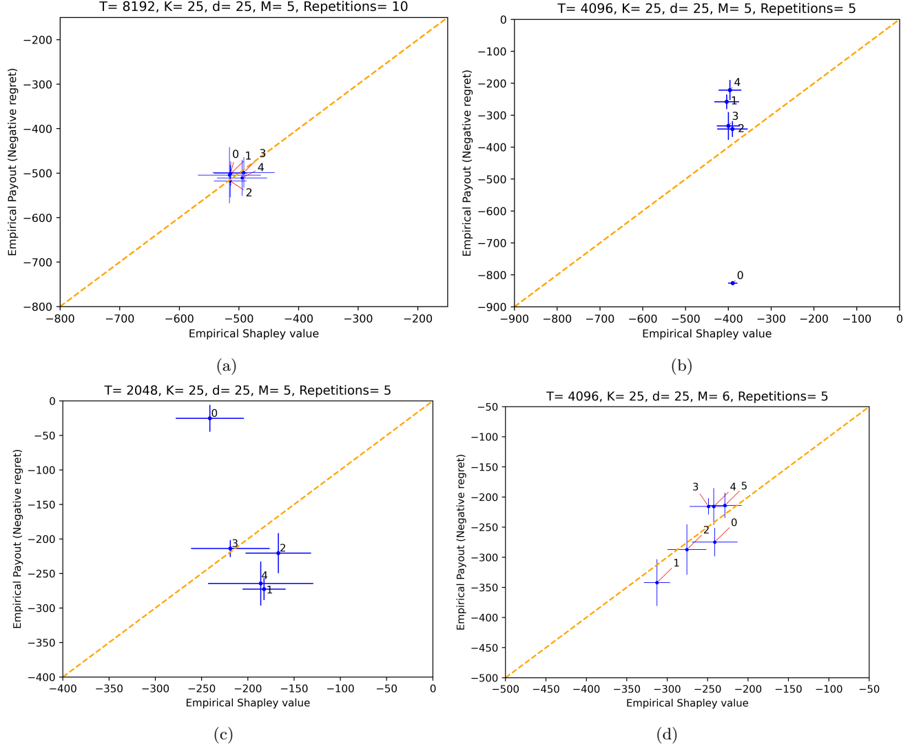
Figure 2: Synthetic experiments
