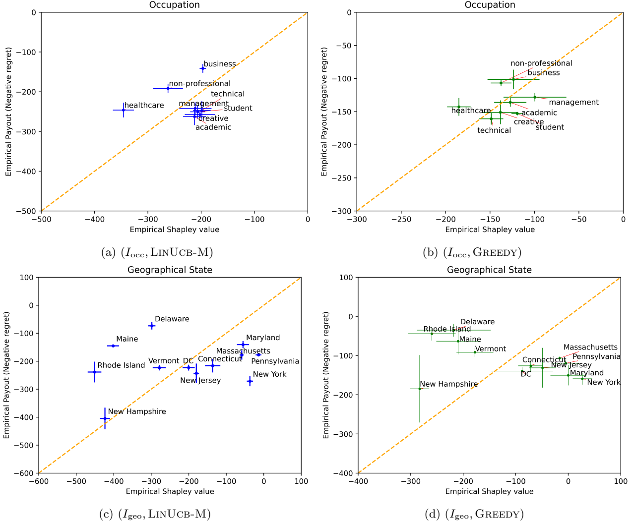
Figure 1: MovieLens experiments
