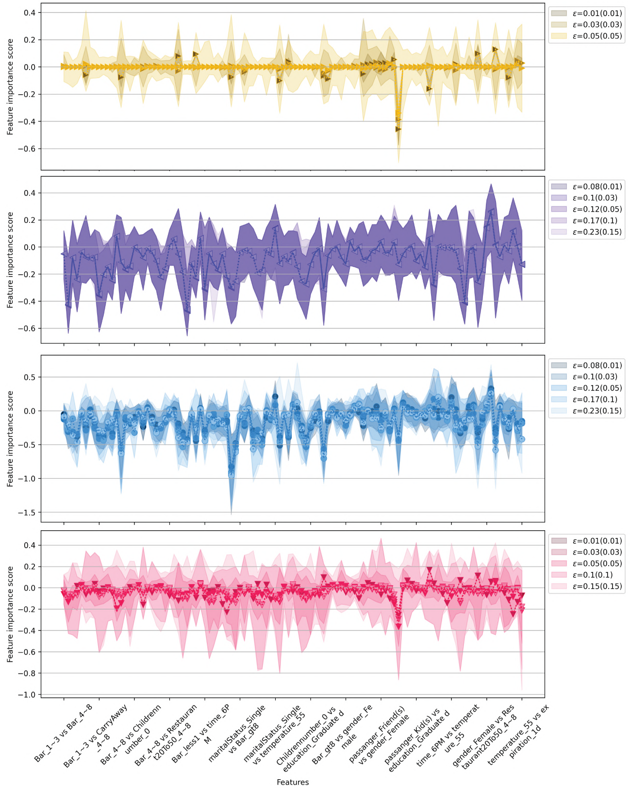
Figure 9: Summary of detailed second-order feature attributions across different methods and epsilons on the dataset BAR, where the x -axis represents features and the y -axis displays feature importance scores. The legend includes epsilons relative to the reference model (in brackets) and to the optimal model identified in practice.
