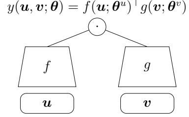
Figure 1: An illustration of the two-tower model, adopted from Yuan et al. (2021).
