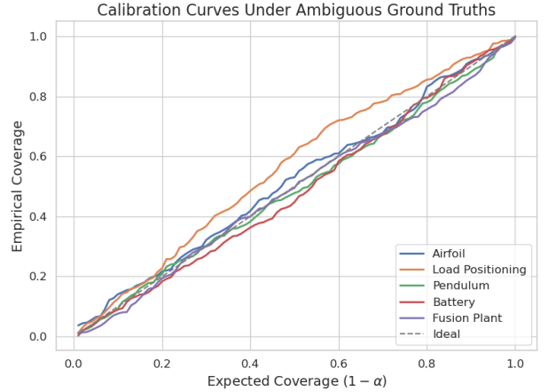
Figure 1: Calibration plots for the tasks, assessed on 1,000 i.i.d. test samples of C with calibration performed using the estimated \tilde{C} , affirming Theorem 3.7.
