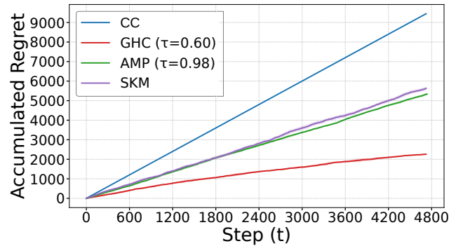
(f) Regret vs. step, E5, ComQA.
