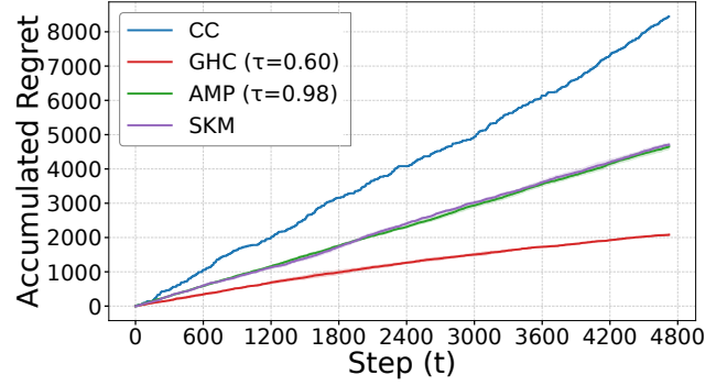
(b) Regret vs. step, Mistral_E5, ComQA.
