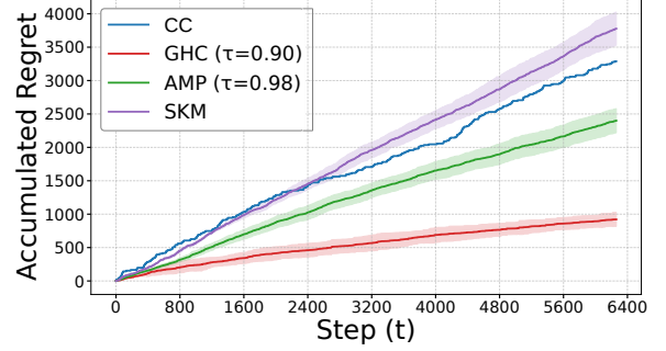
Figure 5: Comparison of different Algorithms on Quora Question Groups dataset with Mistral_E5 .
