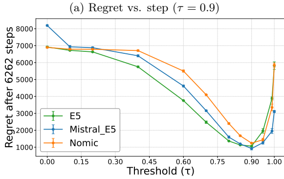
Figure 4: Comparison of GHC using different text embedding models on Quora Question Groups dataset.
