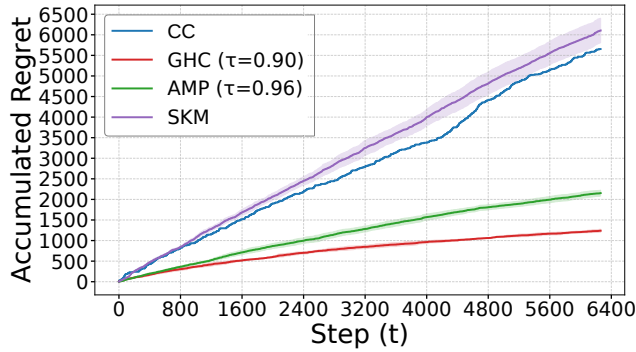
(c) Regret vs. step, Nomic, QQG.
