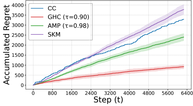
(a) Regret vs. step, Mistral_E5, QQG.
