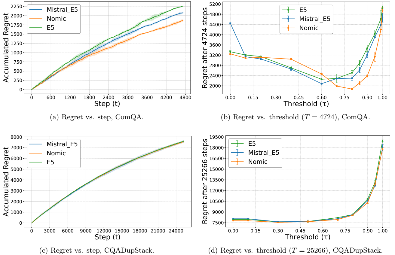
Figure 9: Comparison of GHC with different text embedding models on ComQA and CQADupStack datasets.
