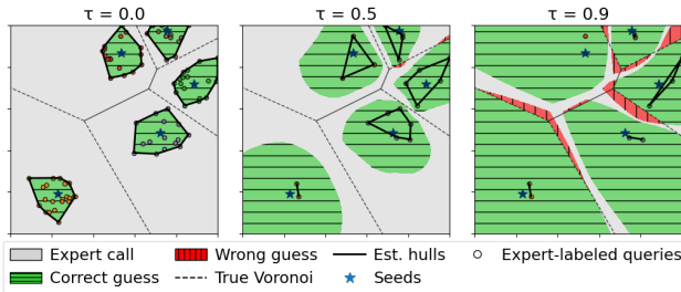
Figure 3: Decision regions of \text{GHC}(\tau) for a mixture of truncated Gaussian distributions, covariance matrix 0.0025I .
