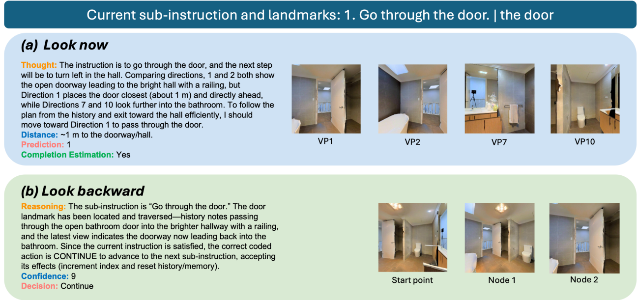
Figure 3: One successful example in the R2R-CE dataset. (a) Look now . Display the current candidate viewpoints and their short descriptions; the MLLM selects the option most aligned with the active sub-goal s_k as the next direction v_t^* . (b) Look backward . Visualize all previously chosen viewpoints to form the executed trajectory \tau ; the MLLM audits \tau against the finished sub-instructions to decide whether the completed sub-goals is satisfied.
