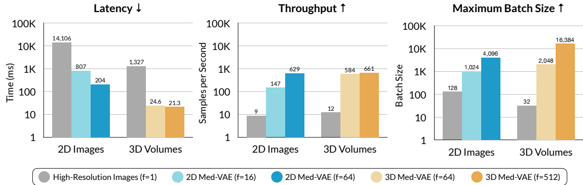
Figure 2: CAD model efficiency. We compare the efficiency of CAD models trained with downsized latent representations to CAD models trained with high-resolution images.
