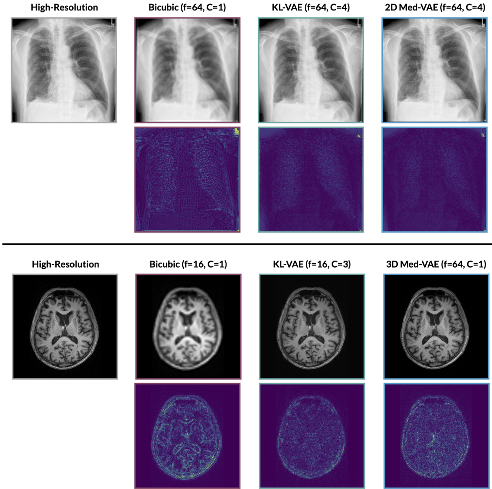
Figure 4: Qualitative examples of reconstructed medical images. The top section provides qualitative examples of a reconstructed chest X-ray. The bottom section provides qualitative examples of a reconstructed brain MRI slice. Residual figures show pixel-level differences between reconstructed images and original, high-resolution images; brighter colors represent larger differences.
