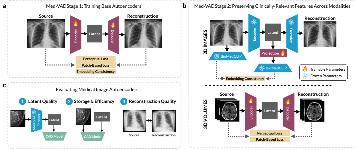
Figure 1: We introduce MedVAE, a suite of large-scale autoencoders capable of downsizing medical images to latent representations and decoding latent representations back to images.
