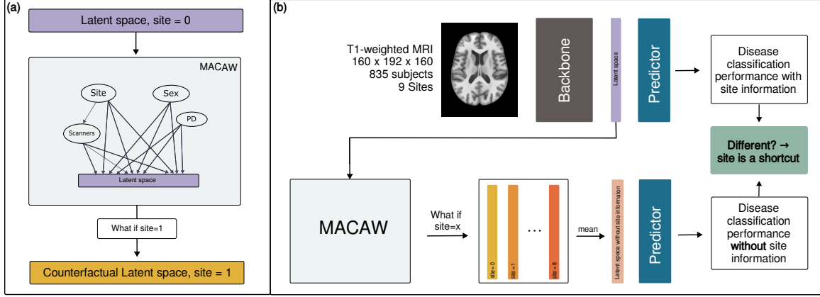
Figure 1: (a) A predefined causal graph was encoded into MACAW to generate counterfactual latents. (b) Counterfactual latents were generated for all sites and then averaged together to remove site-specific information. These site-removed latents were subsequently used for disease classification. If the classification accuracy differs from the standard setup (with site information), it suggests that site information is being used as a shortcut.
