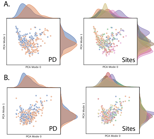
Figure 4: A. PCA modes 0 and 1 of the activation space were visualized based on PD labels and site labels. B. the visualization was then repeated after counterfactually removing site attribute from the activations.
