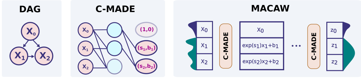
Figure 5: A causal DAG (left) and its respective C-MADE network (center). The MACAW architecture (right) consists of multiple C-MADE networks connected in a series, thereby forming a normalizing flow.
