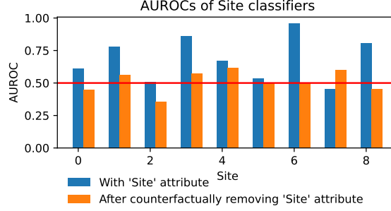
Figure 3: The AUROC for site classification was compared before and after the counterfactual removal of the site attribute.
