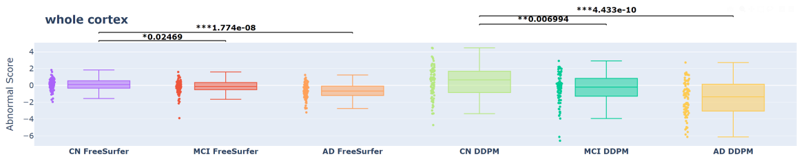
Figure 4: Mean abnormal score across whole cortex The figure shows the distribution comparison between mean abnormal score of the whole cortex per subject for template and DDPM reference sets
