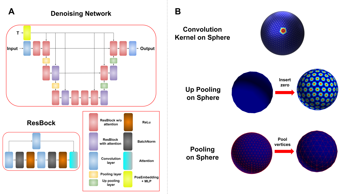
Figure 2: Denoising network structure and operations in spherical domain: (A) A UNet structure with ResBlock built out of spherical convolution, pooling, up-pooling and attention layers. (B) Illustration of spherical operations.
