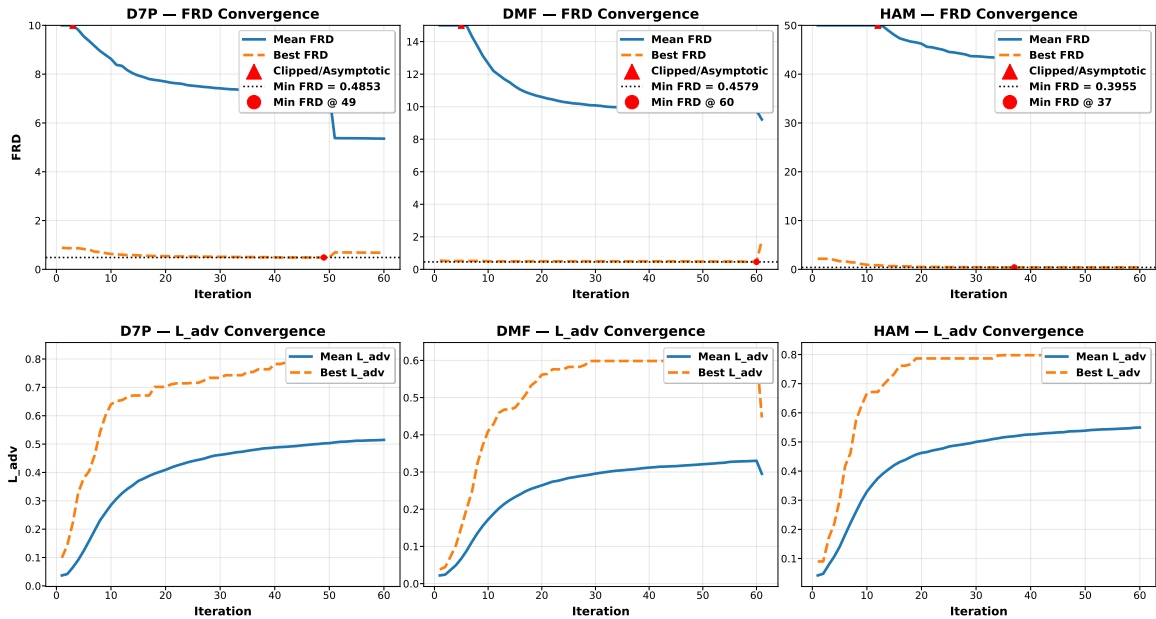
Figure 2: Convergence of minimal FRD and maximal adversarial distance during MOPSO optimization.
