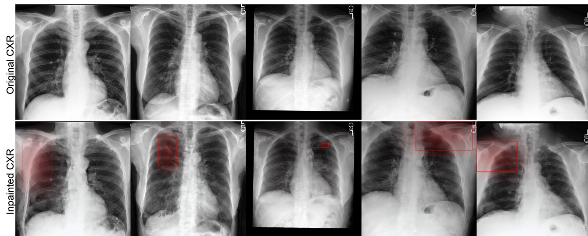
(g) Pneumothorax
