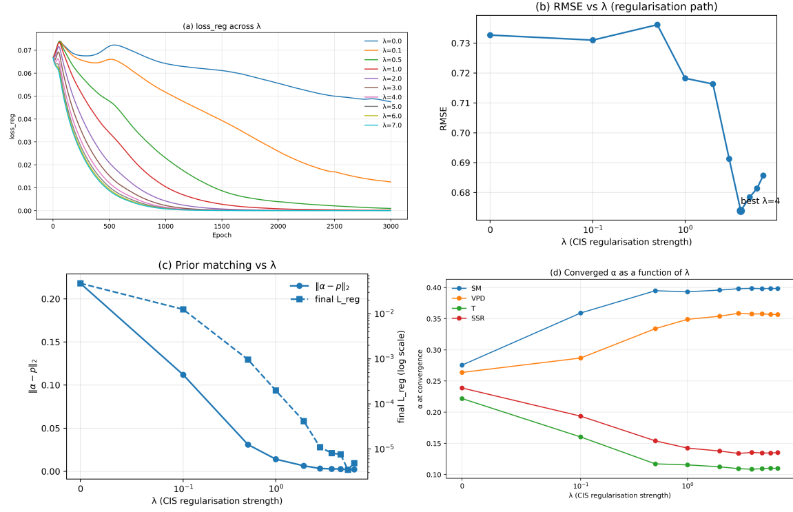
Figure 2: Regularisation and prior alignment of the CIS-guided neural network. (a) CIS regularisation term \lambda L_{\text{reg}} as a function of the regularisation strength \lambda across training. (b) RMSE of predictive performance for the baseline CIS-aware neural network as a function of \lambda . (c) Prior-matching diagnostic \|\alpha - p_{\text{CIS}}\|_2 , illustrating alignment of the learned global feature-gating weights with increasing \lambda . (d) Convergence of the global feature-gating weights \alpha as a function of \lambda .
