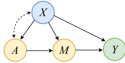
Figure 1: Causal graph. The nodes represent: sensitive attribute, A ; covariate, X ; mediator, M ; target, Y . \rightarrow represents direct causal effect; \dashrightarrow represents potential presence of hidden confounders. 4
