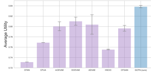
Figure 7: Average utility function value U across different utility weights \gamma on synthetic dataset.
