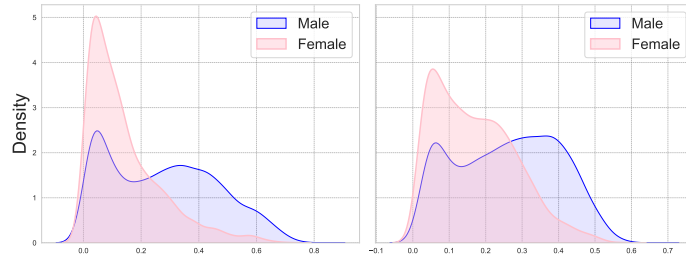
Figure 11: Density plots of the predicted target on the UCI Adult dataset. Left: fairness weight \lambda = 1 . Right: fairness weight \lambda = 5 .
