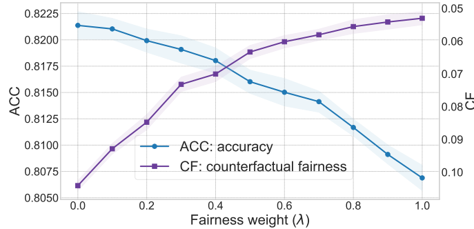
Figure 17: Trade-off between accuracy (ACC) and counterfactual fairness (CF) across different \lambda for a semi-synthetic data. ACC: the higher ( \uparrow ) the better. CF: the lower ( \downarrow ) the better.
