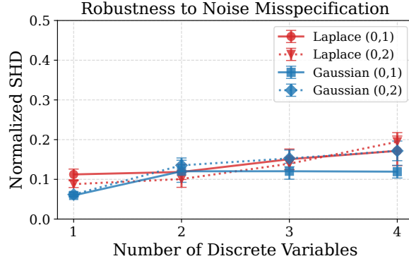
Figure 5: Evaluation of robustness to noise misspecification. Normalized SHD across varying numbers of discrete variables. While our model assumes \text{Laplace}(0, 1) noise, it shows stable performance even when the ground-truth data is generated from Gaussian distributions or different Laplace scale, demonstrating the robustness to noise misspecification.
