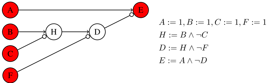
Figure 3: Backup threat canceling
