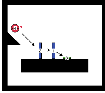
Figure 1: Causal discovery in a chain-reaction system. Directed edges represent causal responsibility rather than low-level physical forces. Holding an object in place breaks the chain reaction and deterministically suppresses all downstream activations, revealing ancestor–descendant relations.
