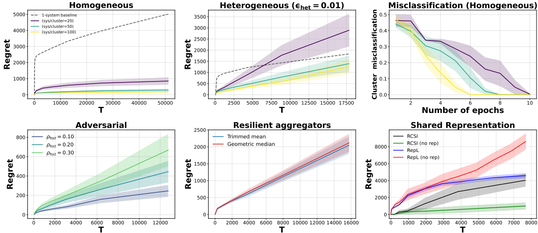
Figure 2: Illustration of main results. Top row: (left) homogeneous clusters; (middle) intra-cluster heterogeneity; (right) misclassification rate. Bottom row: (left) adversarial systems; (middle) robust aggregation comparison; (right) comparison with multitask representation learning.
