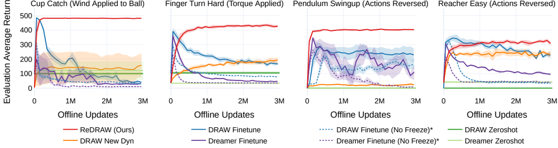
Figure 2: Average evaluation episode return transferring from each DMC environment to a modified variant of it given 40K offline target environment transition samples. Shaded regions indicate the standard error of the mean over 4 seeds for each method. ReDRAW consistently achieves high returns in the target environments and avoids overfitting.
