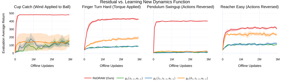
Figure 12: Comparison with a replacement dynamics function g_\psi with the same small capacity as the residual network.
