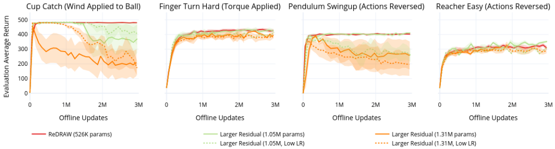
Figure 13: Target environment return during ReDRAW adaptation with larger residual networks. Increasing residual capacity leads to overfitting in later iterations, particularly in Cup Catch and Pendulum Swingup. Reducing the learning rate does not consistently prevent this degradation.
