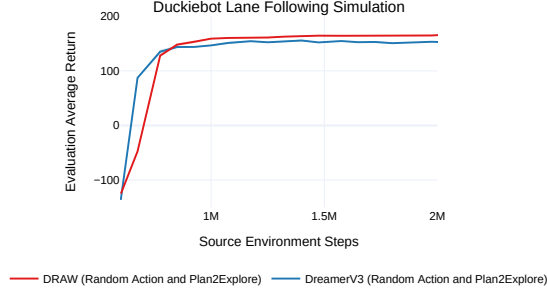
Figure 7: Training curves during pretraining for DRAW and DreamerV3 in the Duckiebot lane following simulation environment. Data collection is performed using random actions for the first 0.6M steps, followed by Plan2Explore for 1.4M steps. Each episode starts from a valid random position. The mean and standard error are shown over 4 seeds.
