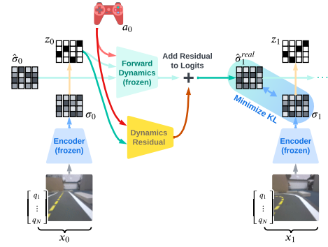
Figure 1: (Left) The DRAW world model is trained to encode states into a discrete latent representation without additional components, from which states, rewards, terminations, and future latent states are predicted. An RL agent can be trained in the world model via synthetic rollouts. (Right) The DRAW world model is frozen. Using a small reward-free dataset, world model dynamics are calibrated to a target environment by training an added residual error correction on latent state dynamics predictions. The RL agent can then be trained under rectified dynamics.
