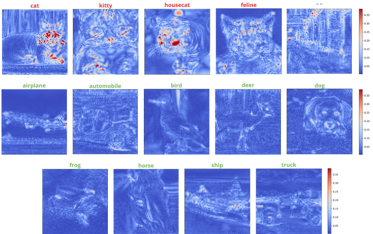
Figure 17: Heatmaps illustrating the differences between noise predictions of the LoRA fine-tuned model and the baseline model for prompts related to cat unlearning. The visualizations include closely related prompts such as “cat”, “kitty”, “feline”, and “housecat”, the neutral prompt “ ”, and prompts corresponding to classes not targeted during unlearning. All heat maps share a common color scale. Differences for the “cat” class and its synonyms are pronounced and localized in key image regions, whereas other classes show much smaller differences. The neutral prompt falls intermediate in difference distribution between the unlearned concepts and the remaining classes.
