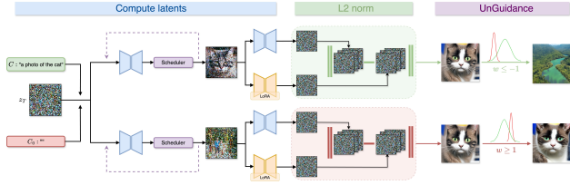
Figure 3: Overview of the adaptive guidance mechanism in UnGuide. We quantify the LoRA adapter’s influence relative to the base model by comparing the norms of predicted noise for a target prompt c and a neutral prompt c_0 . After a short initial denoising phase (typically t = 40 steps), we perform several additional denoising steps ( N = 10 ) to approximate the output distribution. The difference in norms between the base and LoRA model predictions informs adaptive adjustment of the guidance scale: for w \leq -1 , we prioritize the LoRA model to ensure concept erasure (e.g., removing the cat), while for w \geq 1 , we lean on the base model to preserve the original concept in generation.
