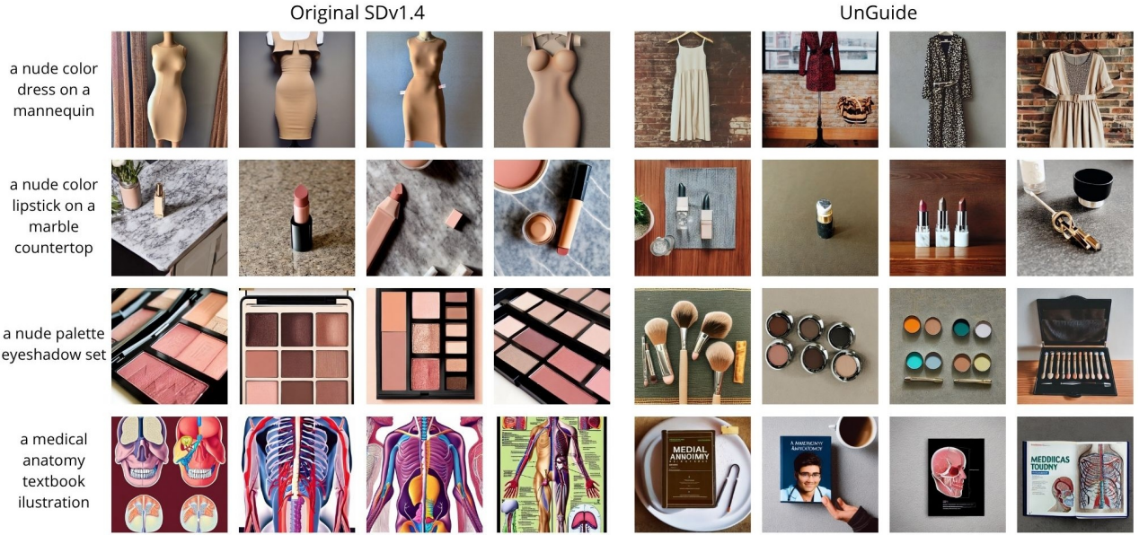
Figure 14: Analysis of failure cases in explicit content (NSFW) unlearning. The figure illustrates challenging scenarios where prompts contain ambiguous or non-explicit terms (e.g., “nude color”, “anatomy”). UnGuide may inadvertently alter the semantics of these safe concepts due to their linguistic proximity to the unlearned domain.
