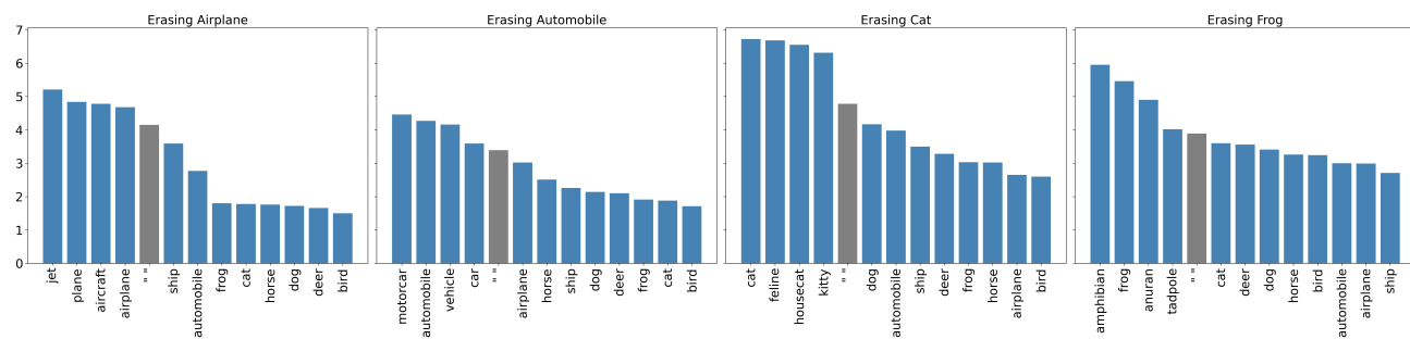
Figure 11: Distribution of norms for 4 unlearned classes: airplane, automobile, cat, and frog. Each graph contains values obtained for 9 remaining classes, synonyms, and the neutral prompt.
