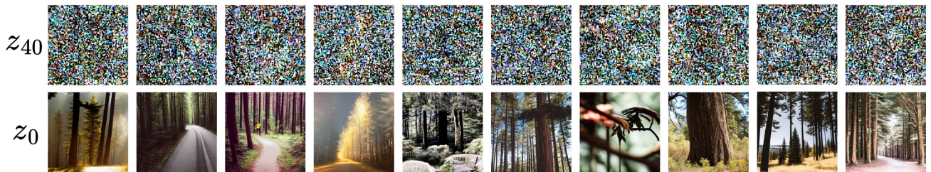
Figure 16: Denoised latent representation ( z_{40} ) of the image, obtained after 10 denoising steps from the the original model, starting from the full noise z_{50} . It is possible to generate additional images from previously obtained latent representations z_t , which were used for noise prediction and L2 norm calculation. The visualization shown assumes a guidance weight of w = -1 and uses z_{40} as starting point for image generation within the UnGuide framework.
