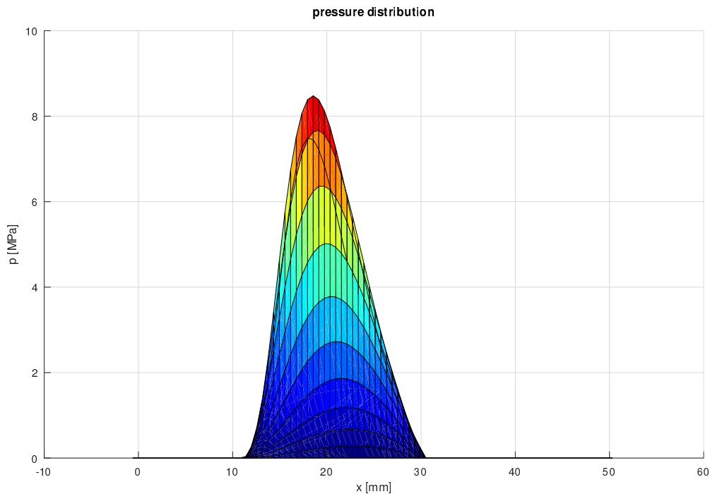
Figure B.1: Pressure distribution in the bearing
