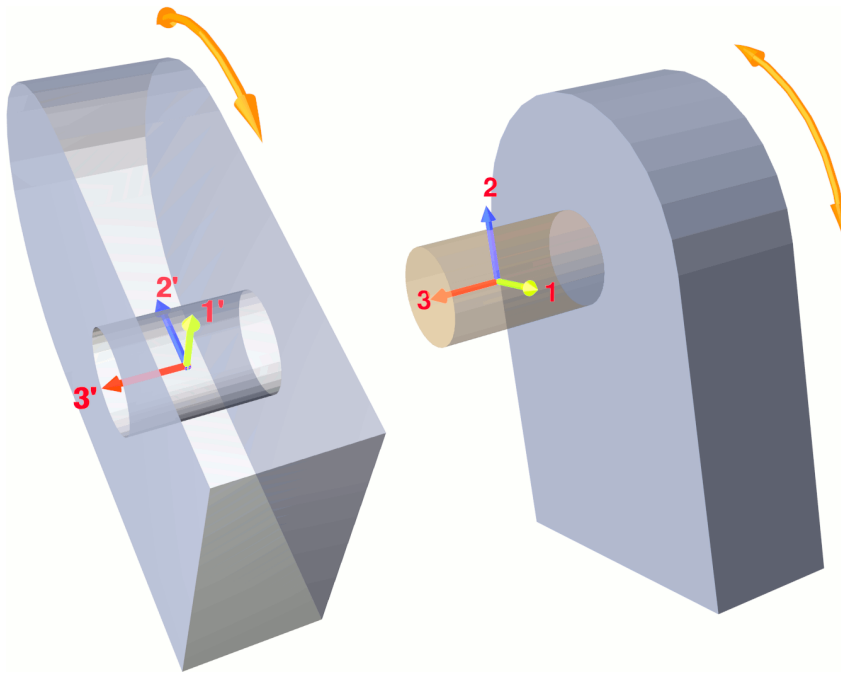
Figure 8.10: Revolute hinge.
