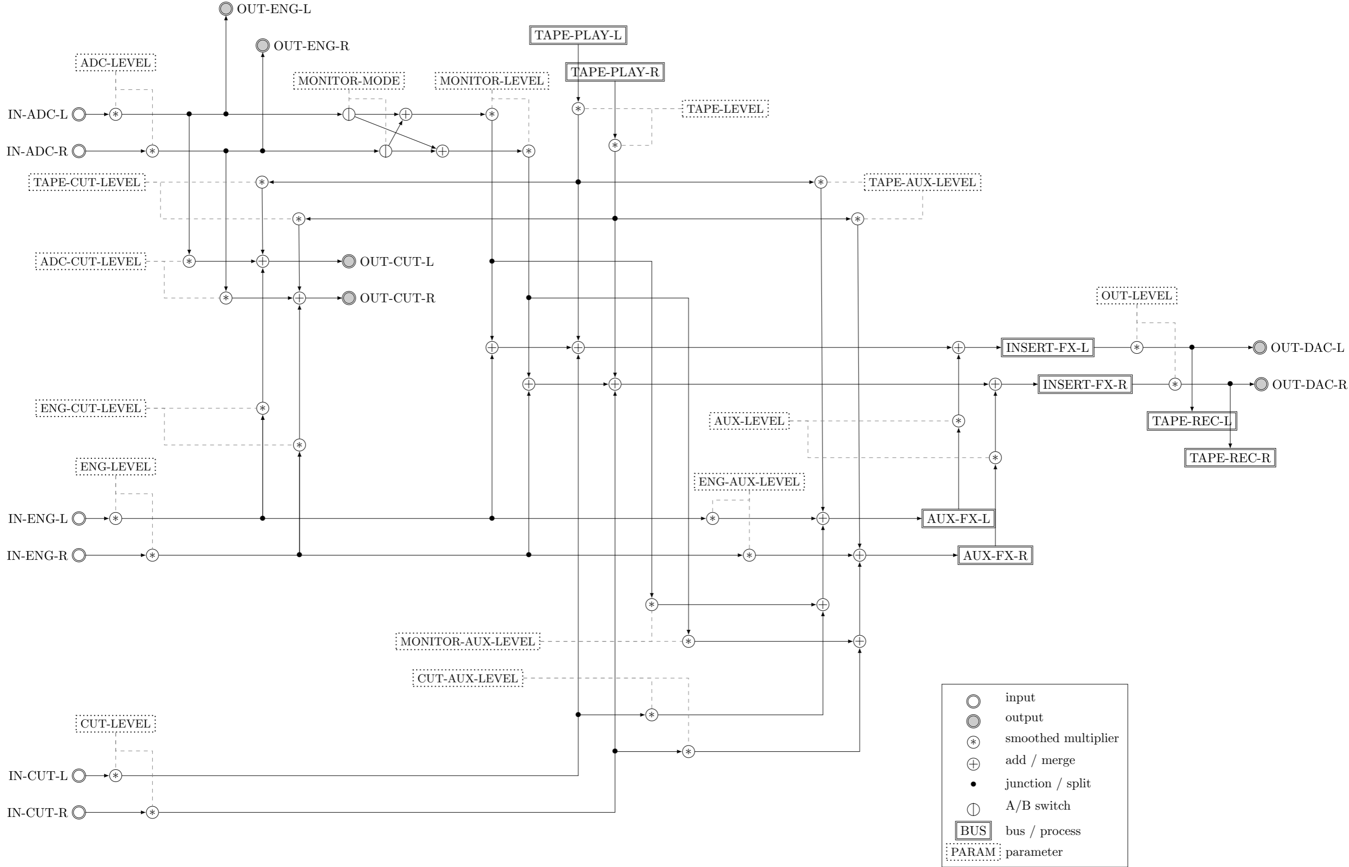
CRONE mixer client, block diagram
